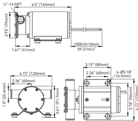
SFSP-01 Impeller, 0.87" (22mm) depth
