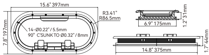
Portlight Profile
