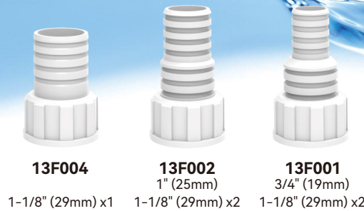
Straight fitting
