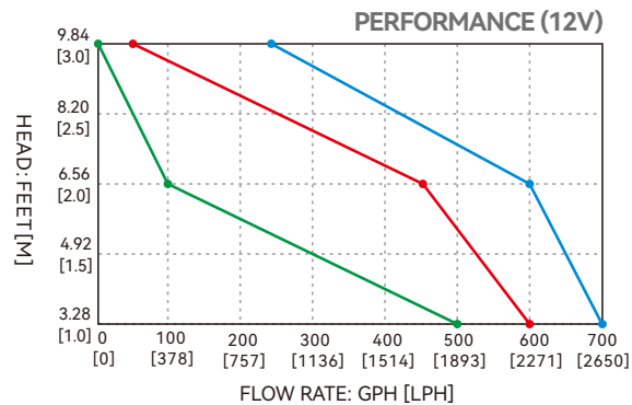
600GPH/2271LPH 800GPH/3028LPH 1100GPH/4164LPH
